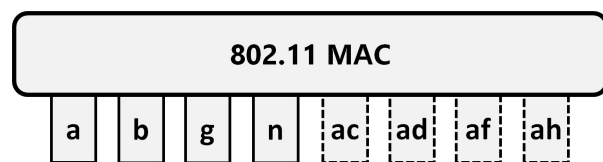
FIGURE 1. One common MAC over multiple PHY options.
