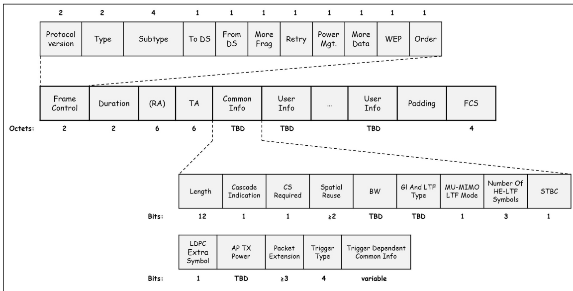
FIGURE 11. Trigger frame format.
