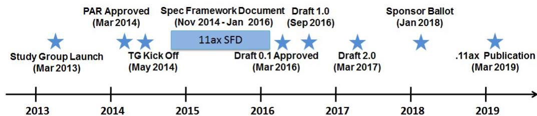
FIGURE 6. 802.11ax timeline.
