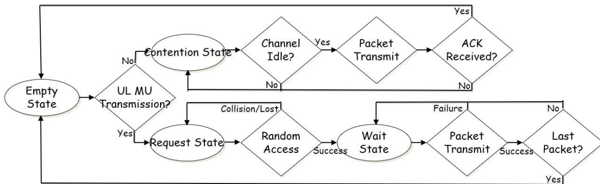
FIGURE 13. HE STA's state transition diagram.
