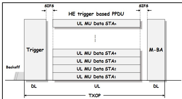
FIGURE 8. An example of UL MU transmission.
