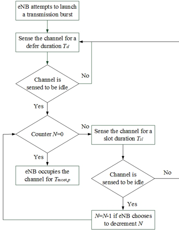
FIGURE 18. Downlink channel access of LAA.
