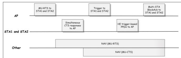
FIGURE 10. An example of MU-RTS/CTS procedure.
