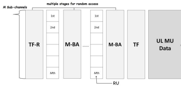
FIGURE 14. IEEE 802.11ax random access protocol.
