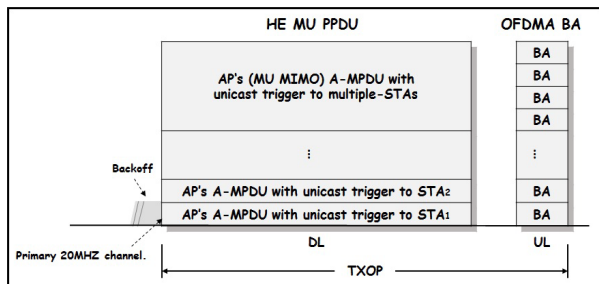
FIGURE 9. An example of DL MU transmission.
